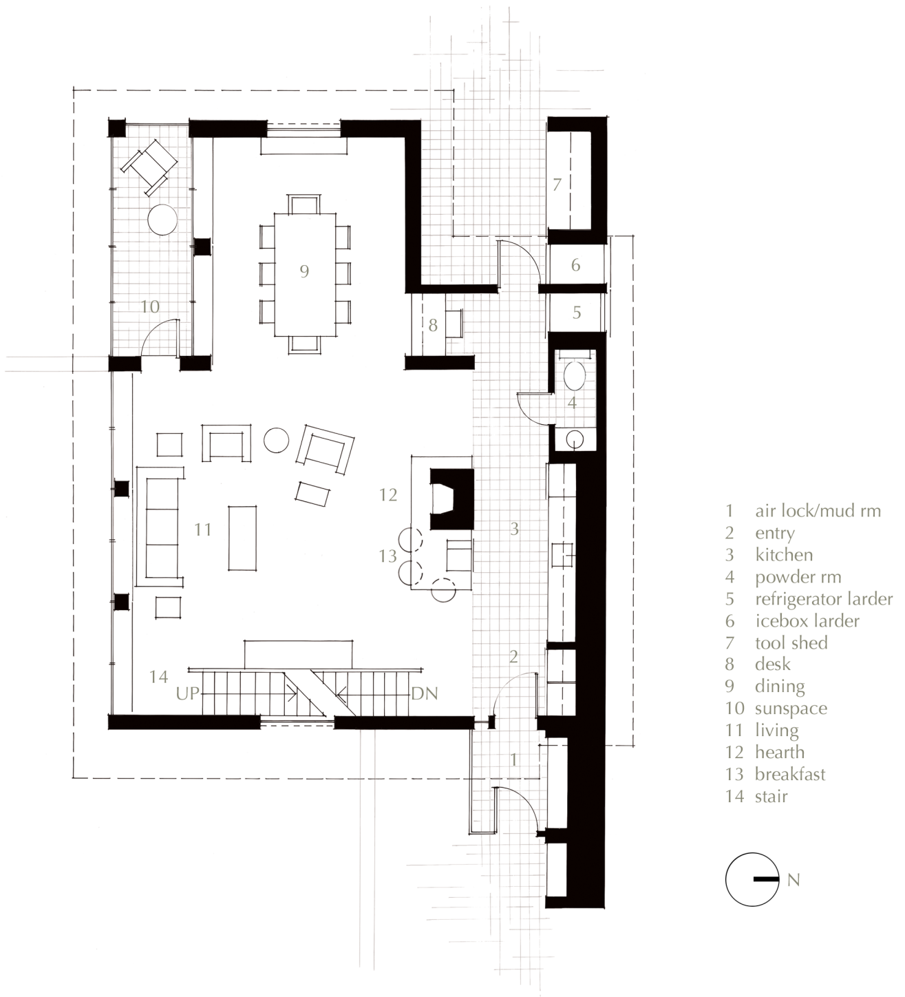
DESIGN A: FIRST FLOOR PLAN
